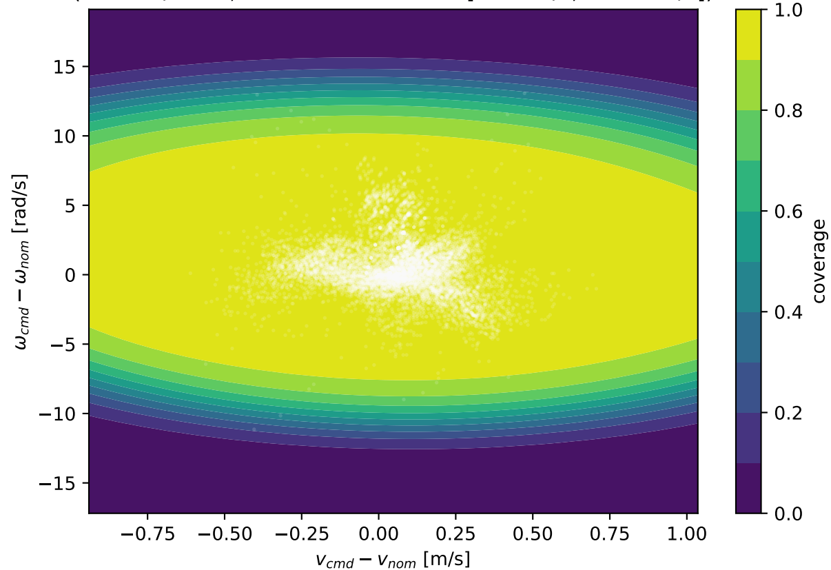
Residual coverage vs command offset (0 = off / OOD; state fixed at mean [0.56 m/s, 0.48 rad/s])
